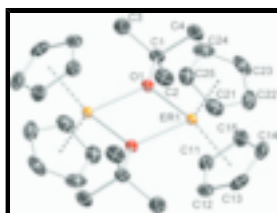
Fig. 1. A view of the title compound showing the atom-labelling scheme. Displacement ellipsoids are drawn at the 50% probability level. H- atoms are omitted for clarity.
